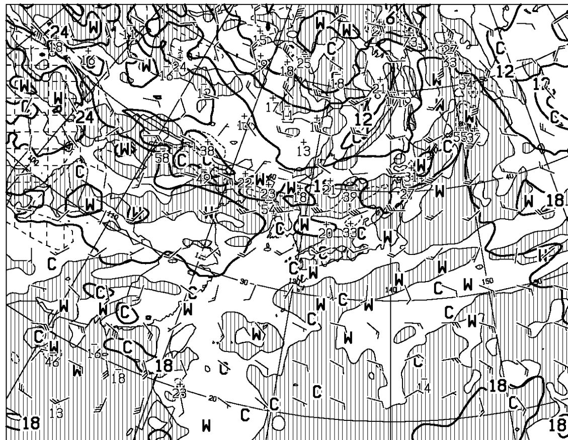
T=24 VALID 090000UTC TEMP (C), WIND ARROW AT 850hPa P-VEL (hPa/h) AT 700hPa
