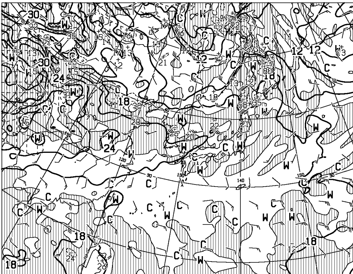
T=12 VALID 081200UTC TEMP (C), WIND ARROW AT 850hPa P-VEL (hPa/h) AT 700hPa
