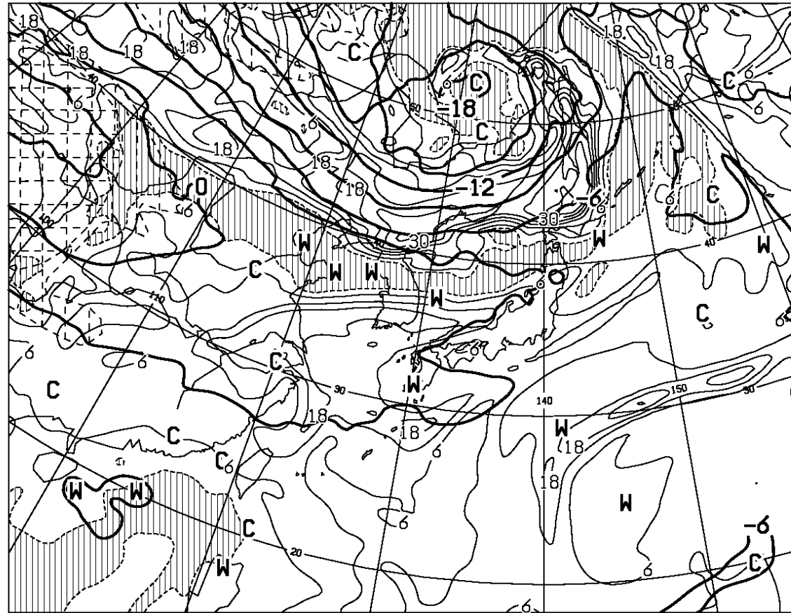
T=24 VALID 090000UTC TEMP (C) AT 500hPa T-TD (C) AT 700hPa
