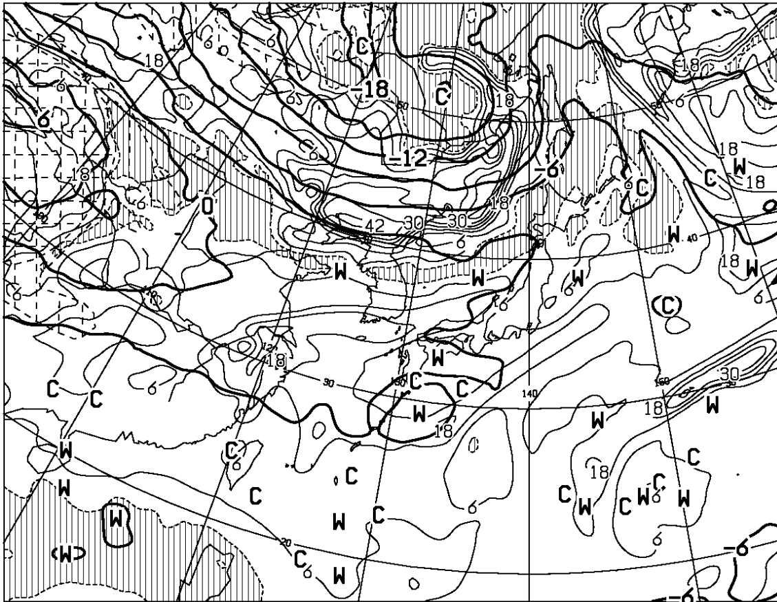
T=12 VALID 081200UTC TEMP (C) AT 500hPa T-TD (C) AT 700hPa
