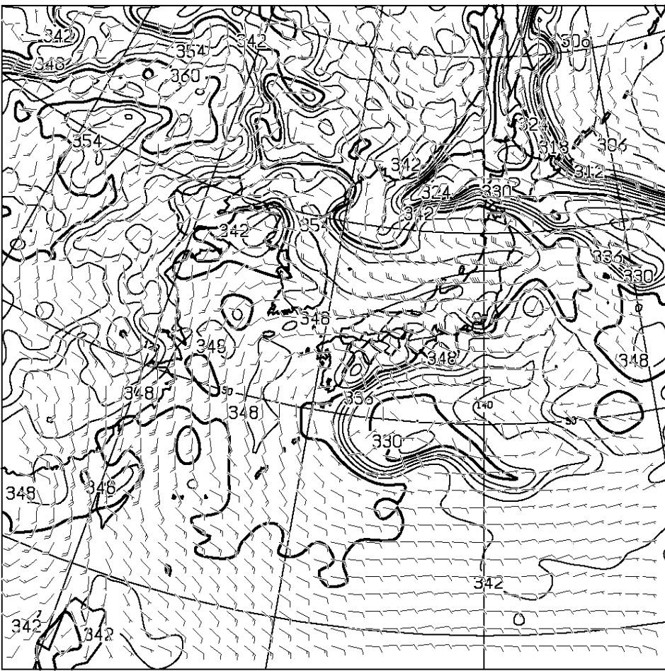
T=36 850hPa: E.P.TEMP(K),WIND(KNOTS) VALID 031200UTC
