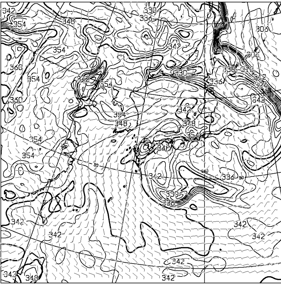
T=12 850hPa: E.P.TEMP(K),WIND(KNOTS) VALID 021200UTC
