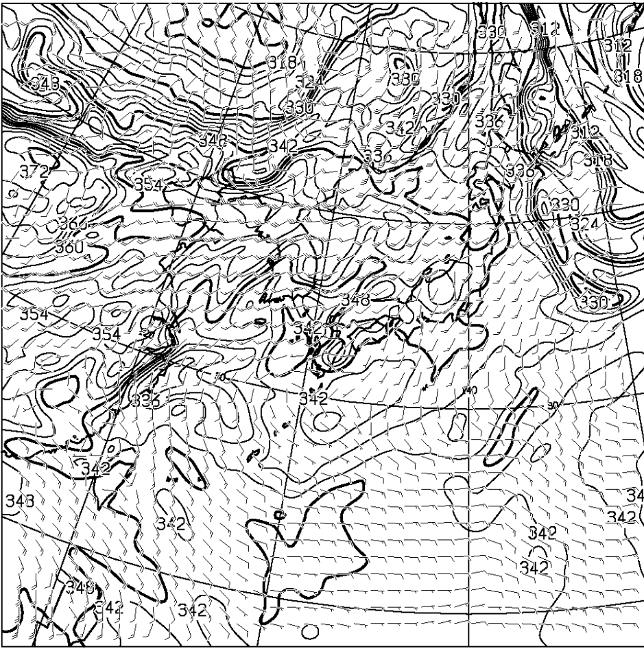
T=12 850hPa: E.P. TEMP(K), WIND(KNOTS) VALID 071200UTC
