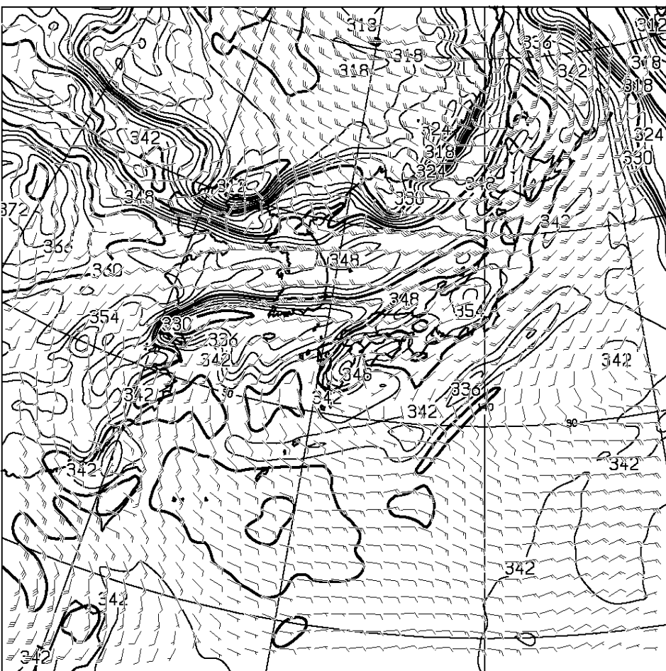
T=36 850hPa: E.P. TEMP(K), WIND(KNOTS) VALID 081200UTC
