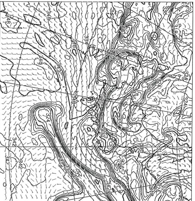
T=36 850hPa: E.P. TEMP(K), WIND(KNOTS) VALID 020000UTC
