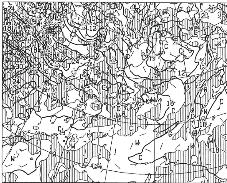
T=48 VALID 021200UTC TEMP(O), WIND ARROW AT 850hPa P-VEL(hPa/h) AT 700hPa
