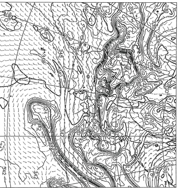
T=48 850hPa: E.P. TEMP(K), WIND(KNOTS) VALID 021200UTC
