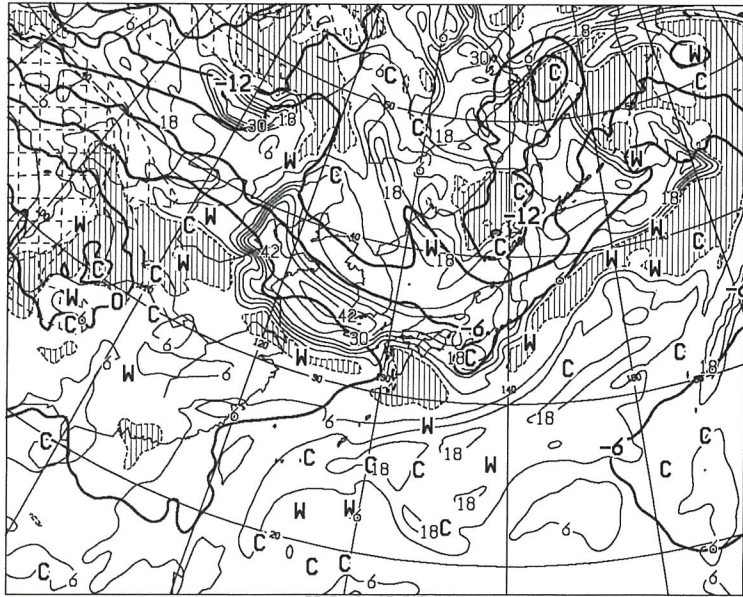
T=36 VALID 020000UTC TEMP(C) AT 500hPa T-TD(C) AT 700hPa
