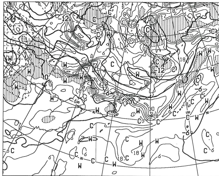
T=48 VALID 021200UTC TEMP(C) AT 500hPa T-TD(C) AT 700hPa
