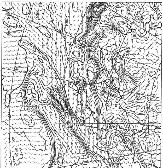
T=12 850hPa: E.P. TEMP(K), WIND(KNOTS) VALID 010000UTC
